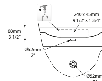
Rim Detail
