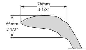
Rim Detail
